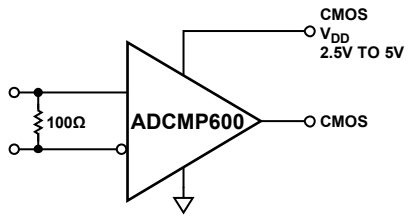
Figure 23. LVDS-to-CMOS Receiver
