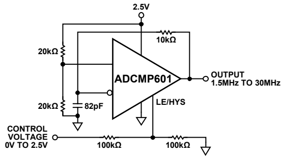
Figure 24. Voltage-Controlled Oscillator
